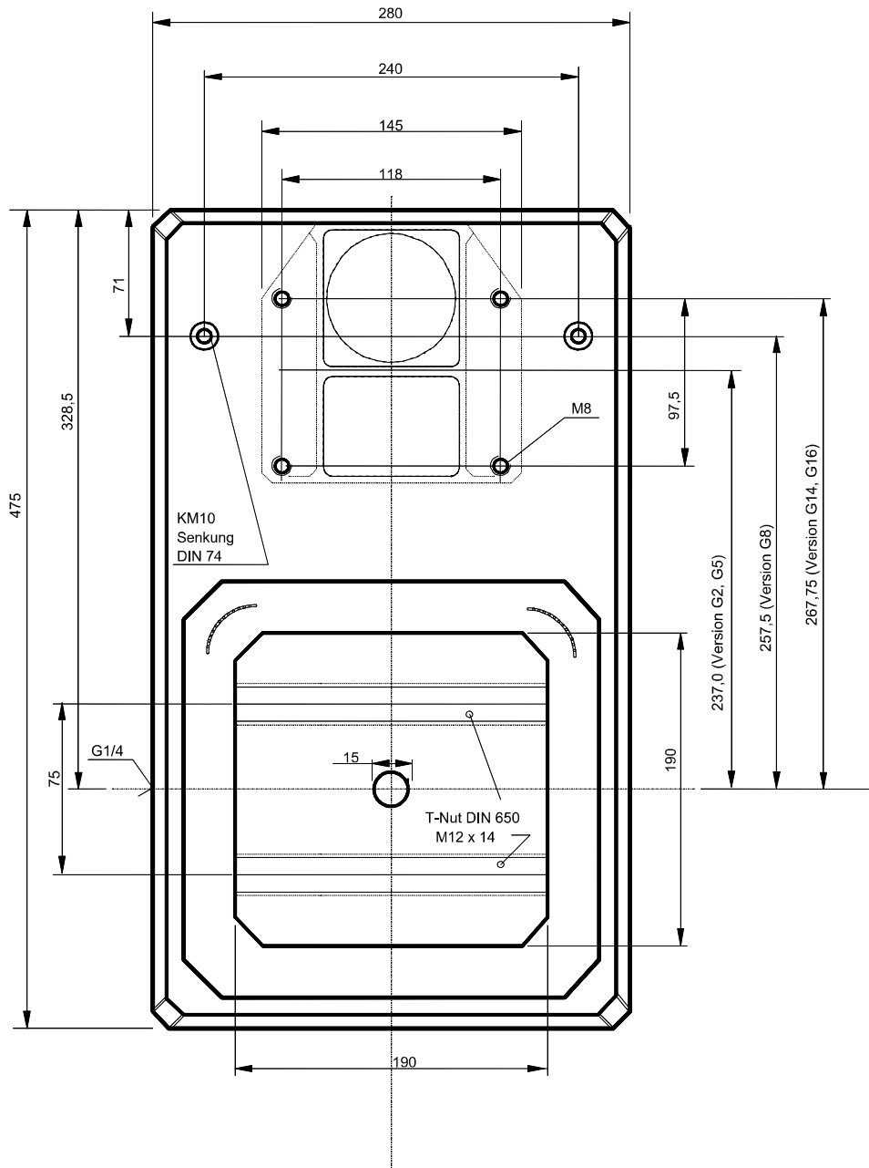
Dimensions of the base plate
